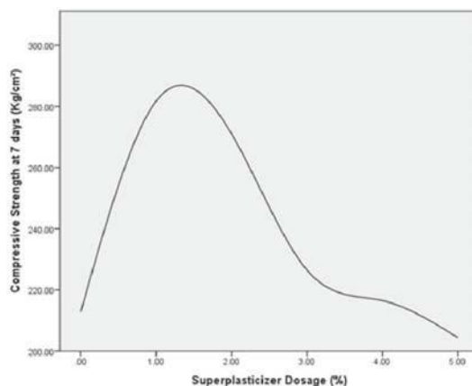
Fig. 3 Compressive strength at 7 days for different dosages of superplasticizer
