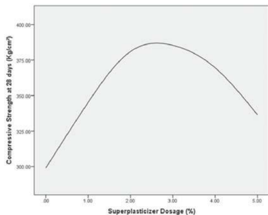
Fig. 2 Compressive strength at 28 days for different dosages of superplasticizer
