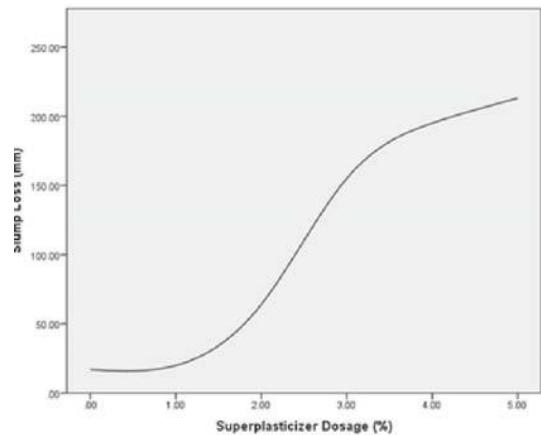
Fig. 1 Slump test results at different superplasticizer dosages
